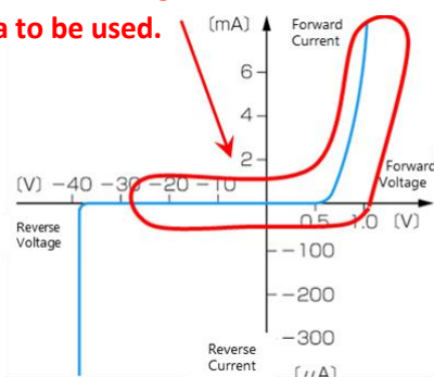
Current vs. Voltage Characteristics of Switching Diodes
