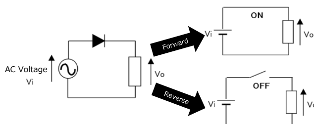
Forward and reverse voltage operation
